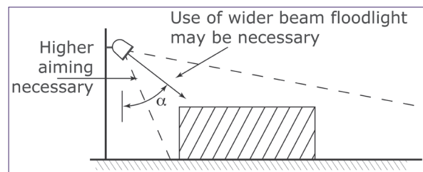
✗ Figure 3: Lower mounting height – more spill light and glare
