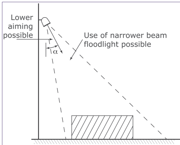
✓ Figure 2: Higher mounting height – less spill light and glare
